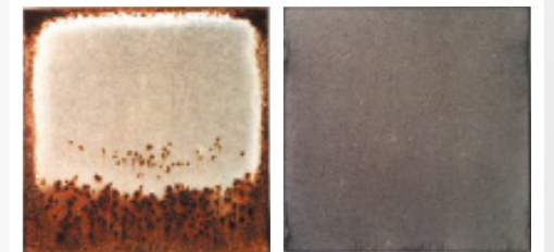
Galvanised steel Z275 (Heavy sign of Rust) ZINCALUME® steel (No Sign of Rust)
